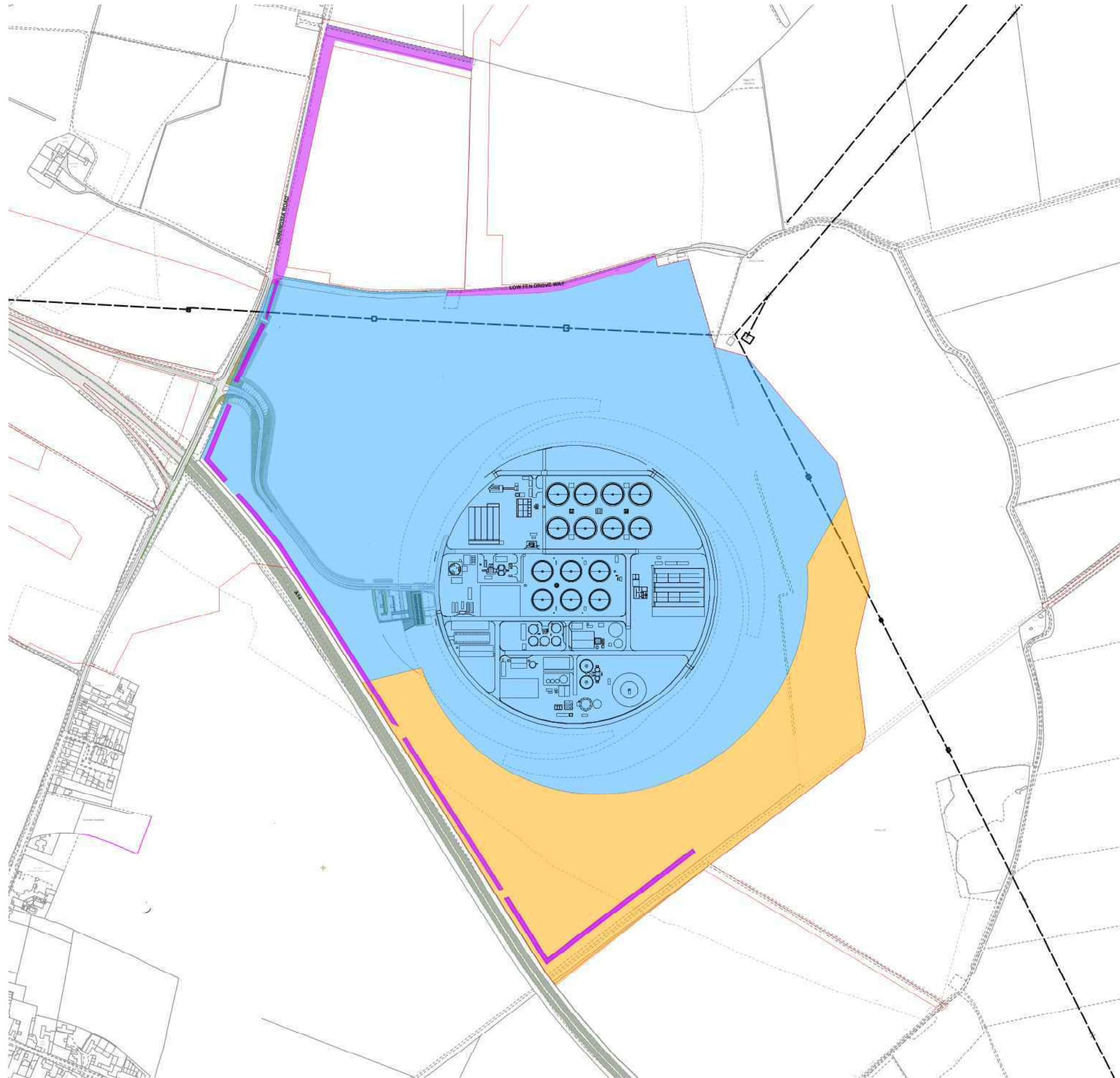
Figure 3.3 Phasing Plan
